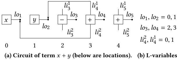
Figure 4: Encoding via integer location variables.
